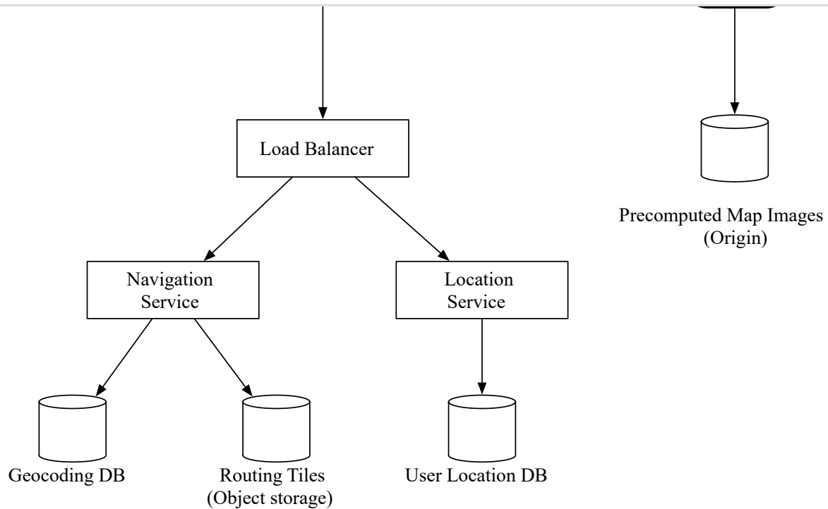
Figure 7 High-level design
