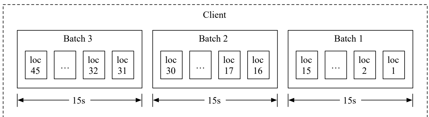
Figure 9 Batch requests
