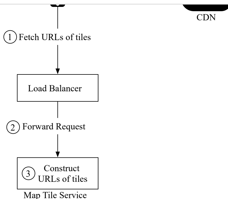
Figure 12 Map rendering
