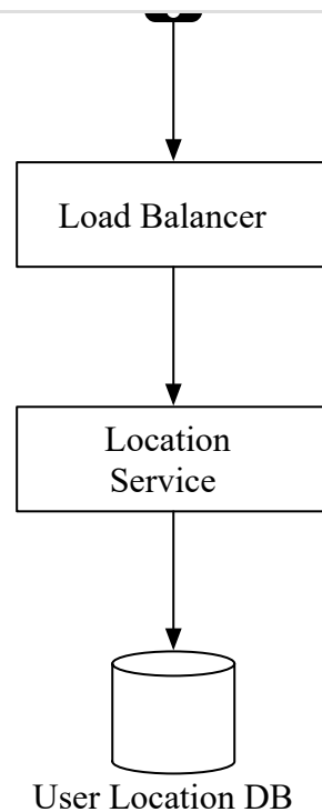
Figure 8 Location service
