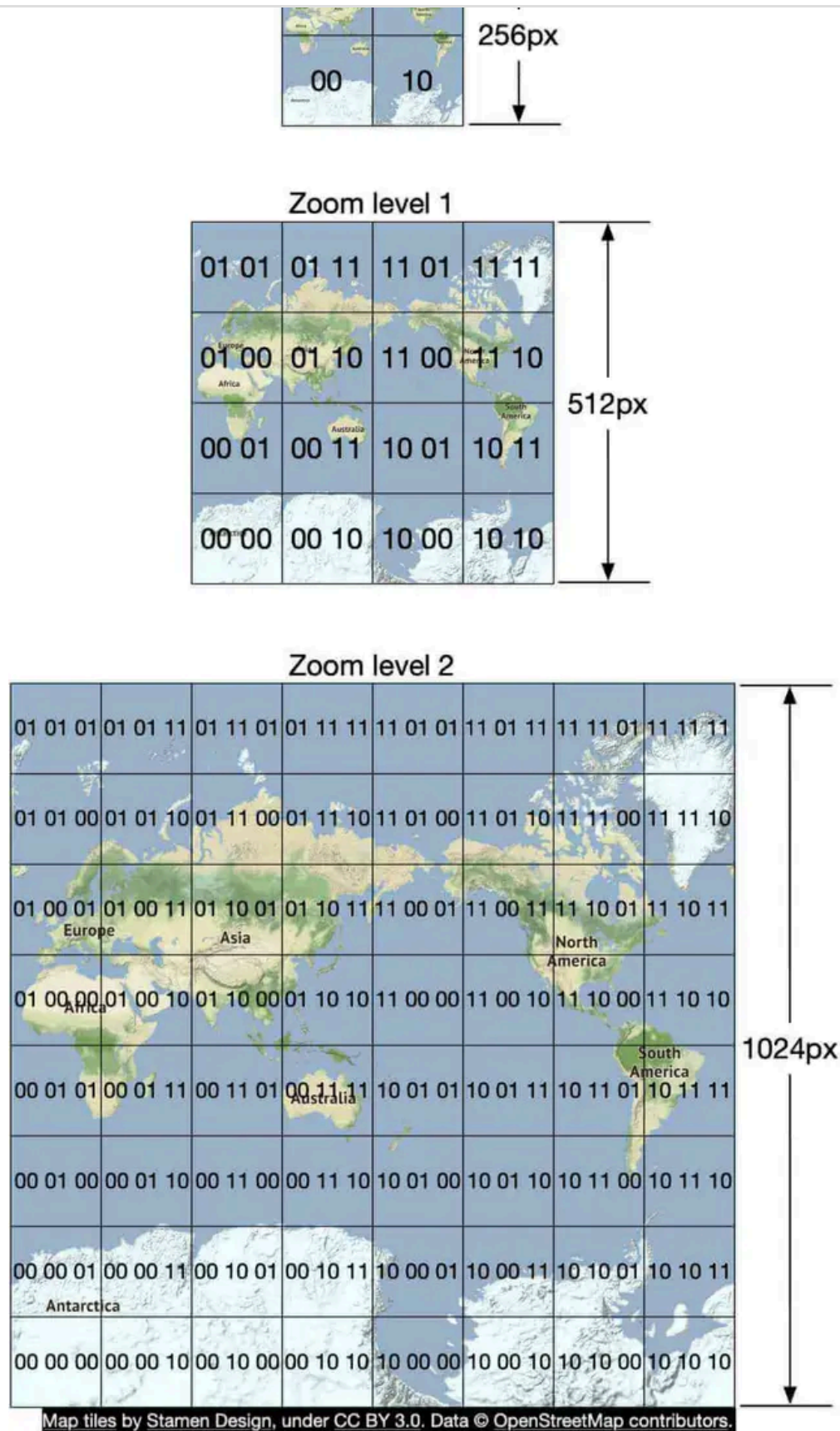
Figure 16 Zoom levels
