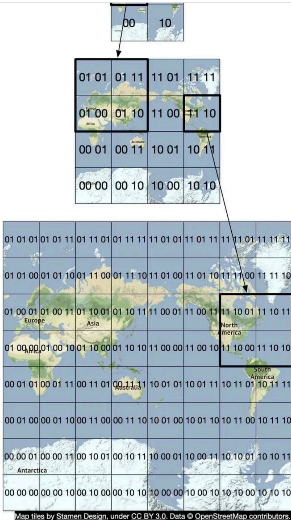
Figure 3 Geohashing
