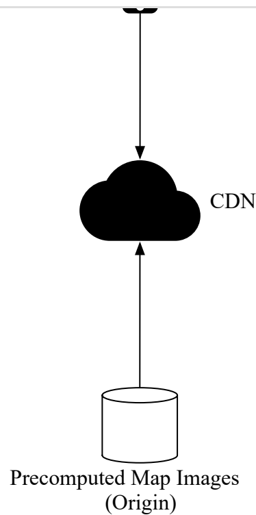
Figure 10 CDN
