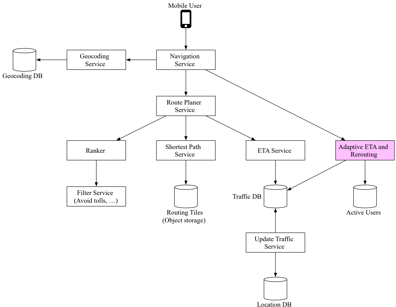
Figure 21 Final design
